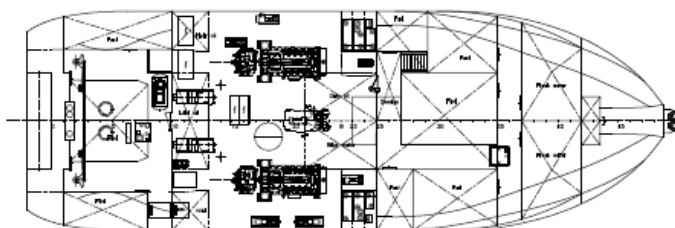
Below maindeck
