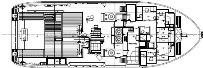
Below maindeck
